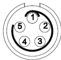
P4 plug welding surface
